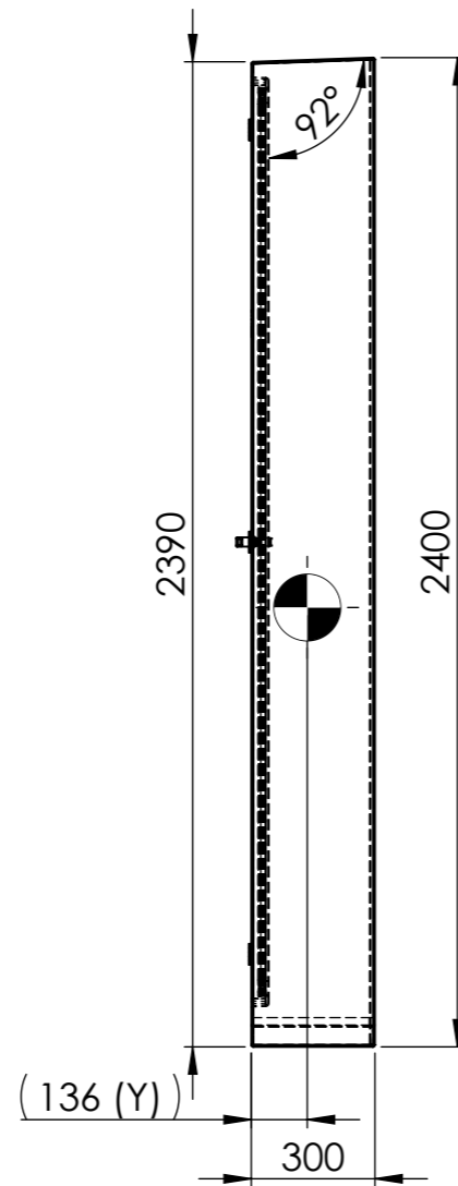
Side View
