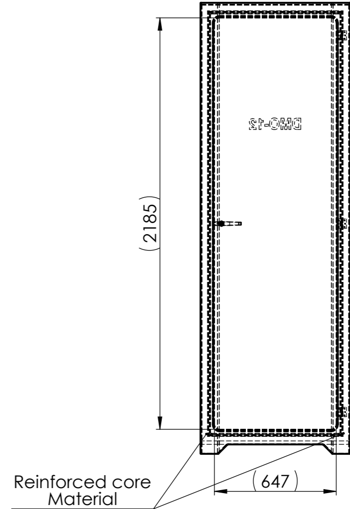
Rear View
